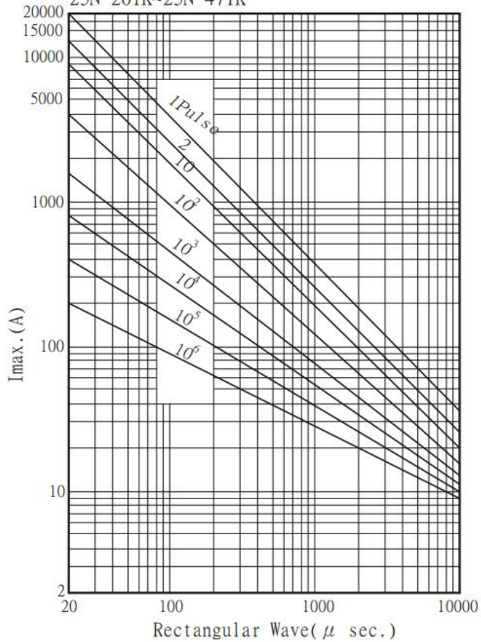
Pulse Life time Ratings -25mm 25N 201K~25N 471K
